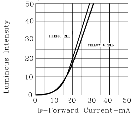
Luminous Intensity VS. (mcd) Forward Current
