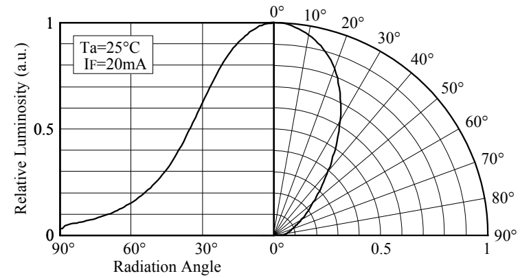
■ Directivity (NSPW315BS)
