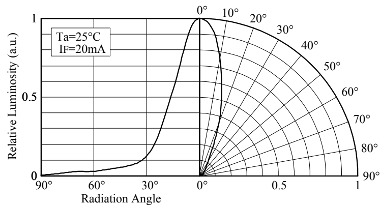
■ Directivity (NSPW312BS)
