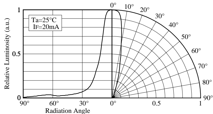
■ Directivity (NSPW300BS)
