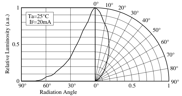
■ Directivity (NSPG320BS)
