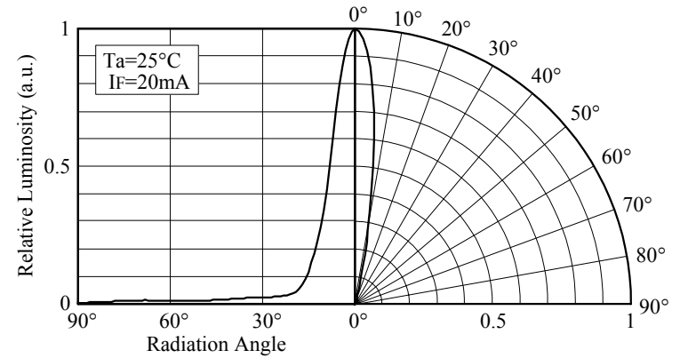
■ Directivity (NSPB500(S))
