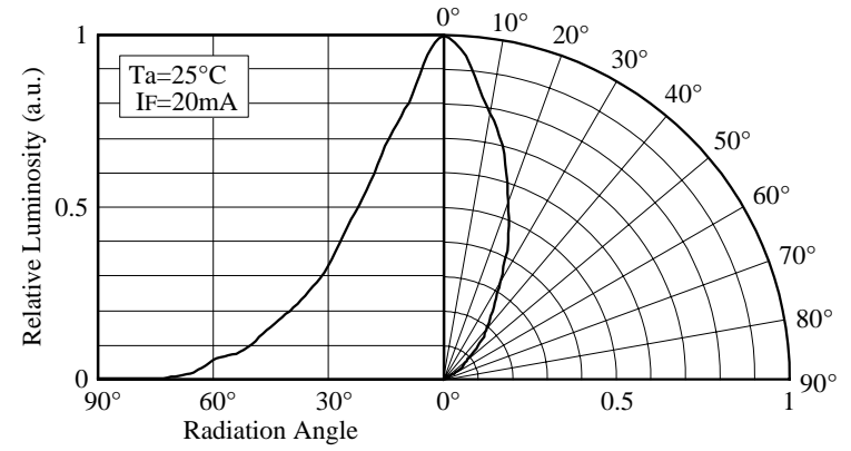
■ Directivity (NSPB320BS)
