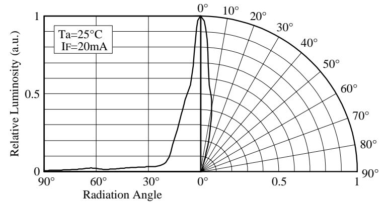
■ Directivity (NSPB300A)
