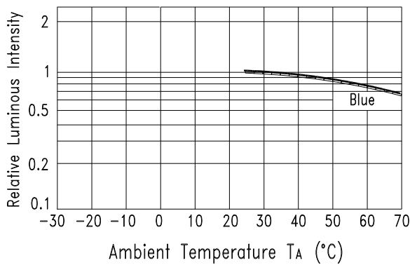
Fig.5 Luminous Intensity vs. Ambient Temperature T_A (°C)
