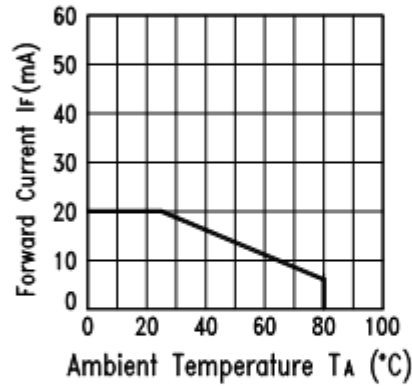
Fig.3 Forward Current Deratina Curve
