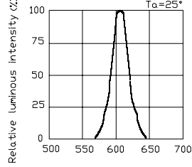
Spectrum Distribution
