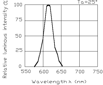
Spectrum Distribution Ta=25°
