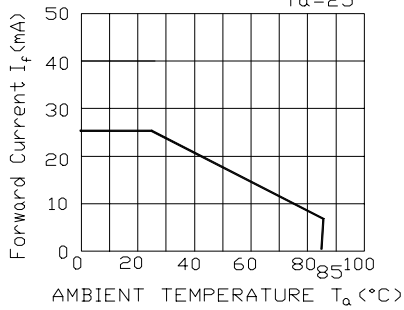
Forward Current Derating Curve Ta=25°
