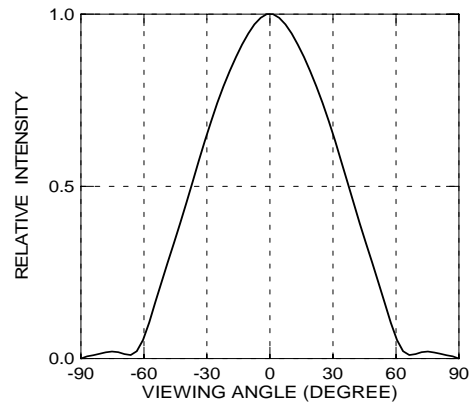
Relative Intensity vs. Off Axis Angle
