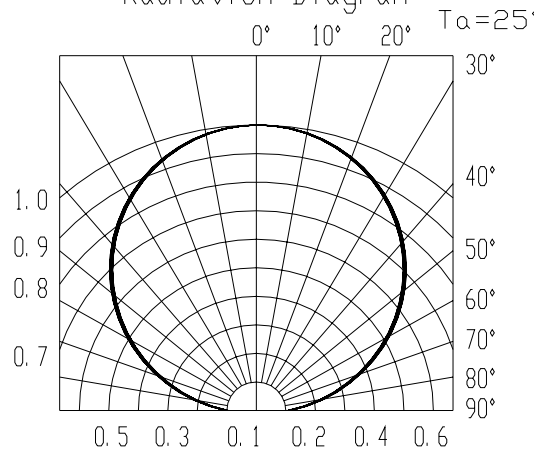
Radiation Diagram
