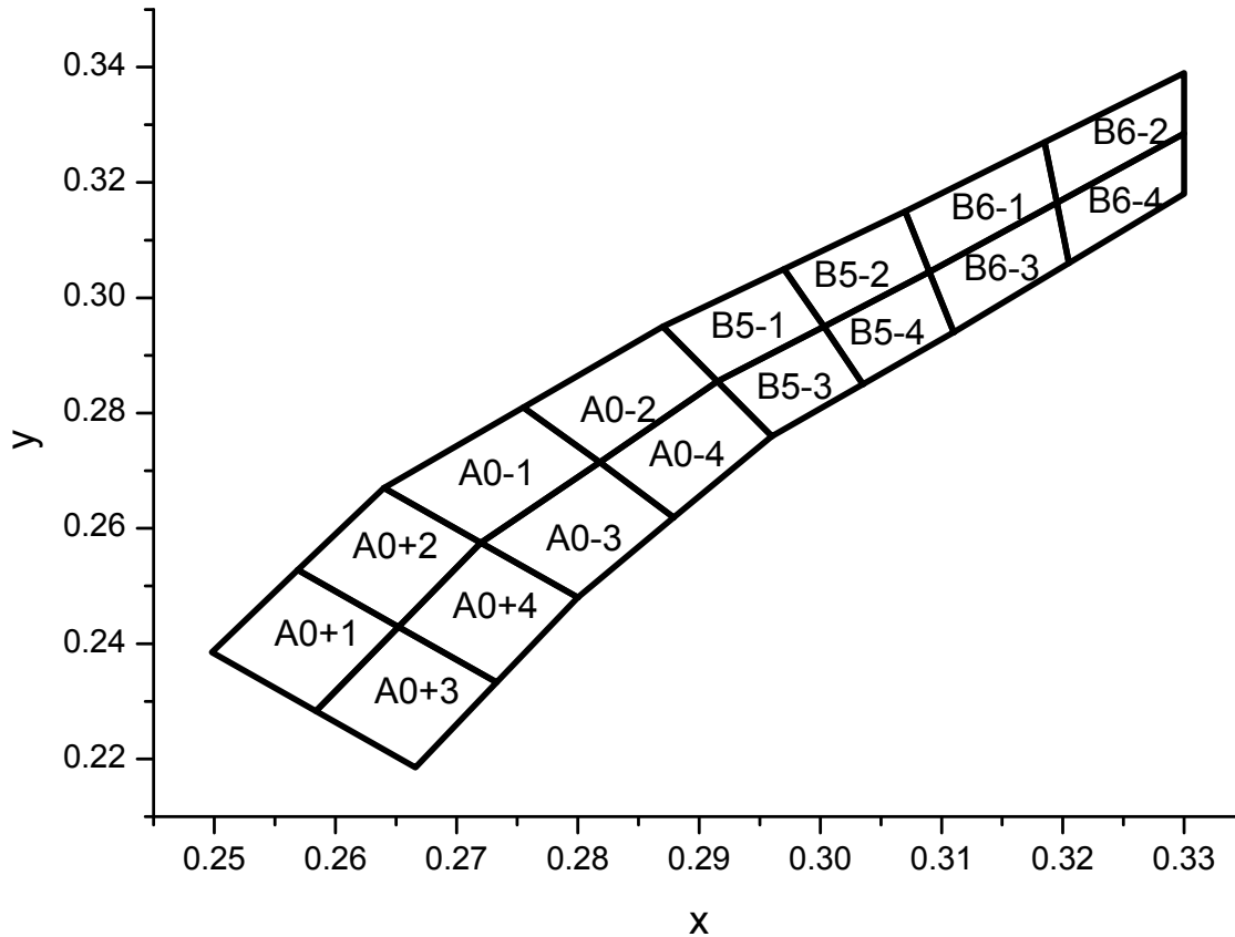
The C.I.E. 1931 Chromaticity Diagram
