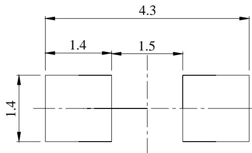
Recommended soldering pad design
