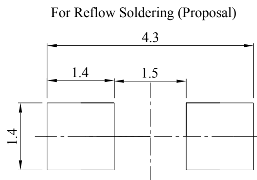
Recommended soldering pad design
