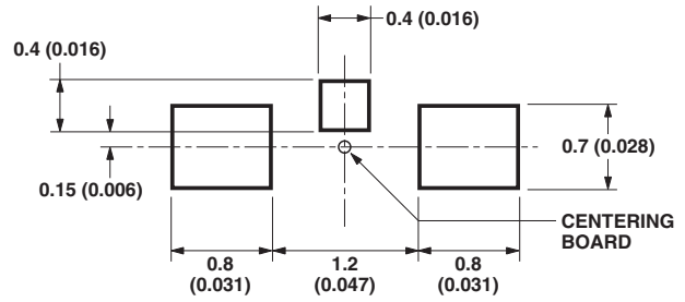
Figure 11. Recommended soldering pattern for HSMx-C120.
