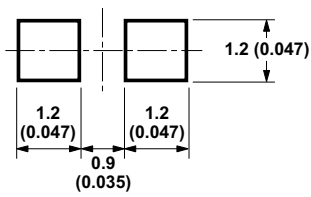
Figure 12. Recommended soldering pattern for HSMx-C170.
