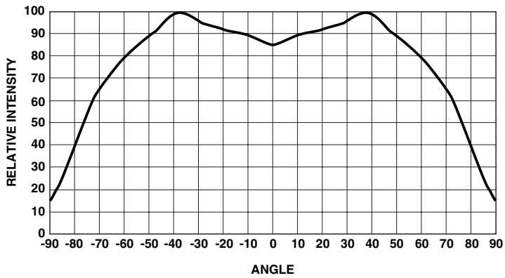
Figure 5. Relative intensity vs. angle for HSMx-C120.
